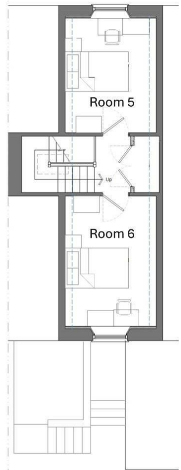
Third Floor
